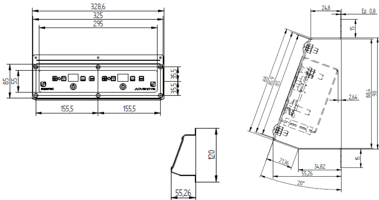
Control panel frame (option/not included)
