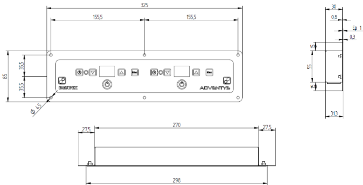
Cut-out dimensions lexan control panel
