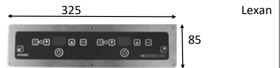
Control cut out dimensions 302 x 60mm
